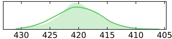
Intrusive 0
